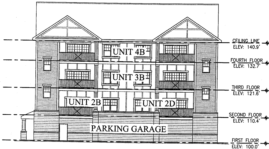
WEST ELEVATION
