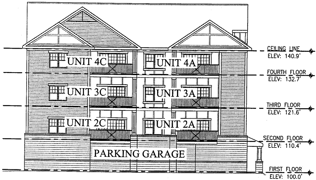
EAST ELEVATION
