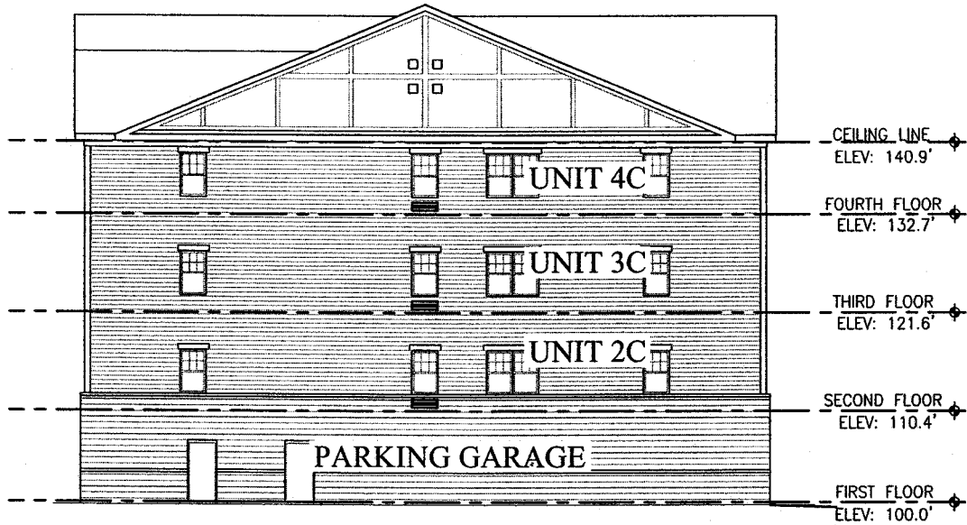
SOUTH ELEVATION
