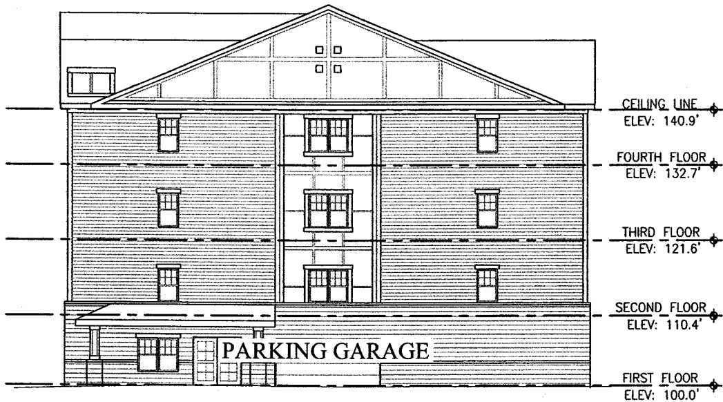
NORTH ELEVATION
